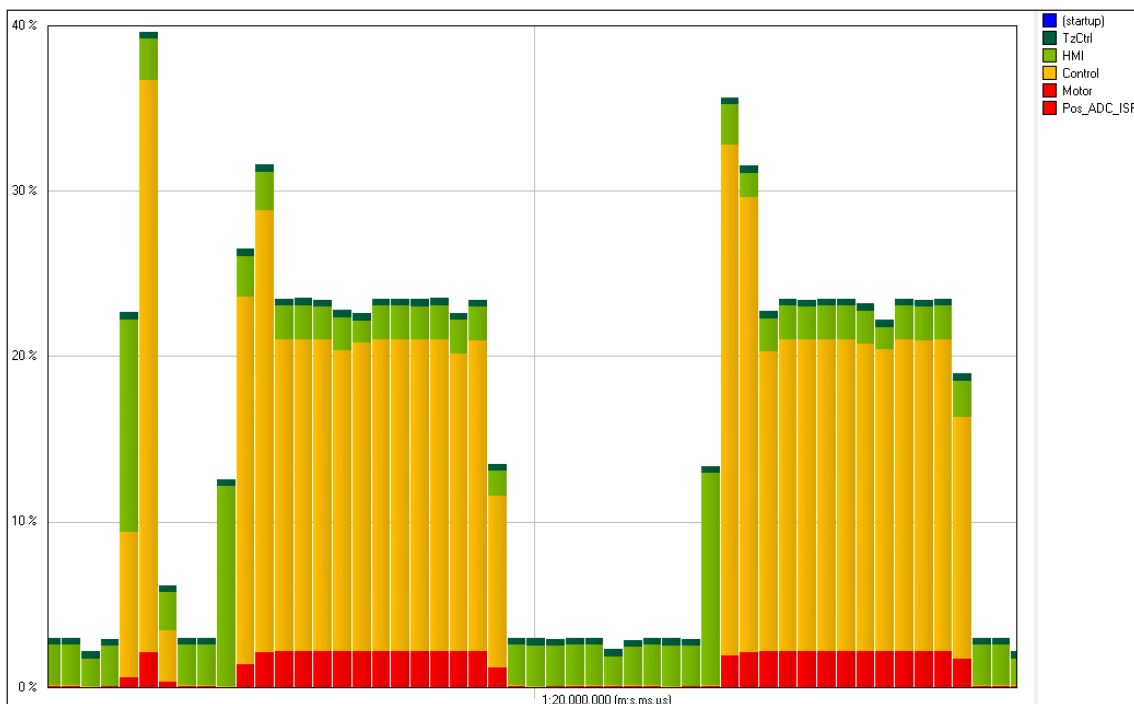
A CPU load graph from Percepio Tracealyzer shows processor usage per task over time, clearly showing where a specific task is consuming much higher CPU resources than others.
